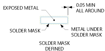
SOLDER MASK DETAILS
